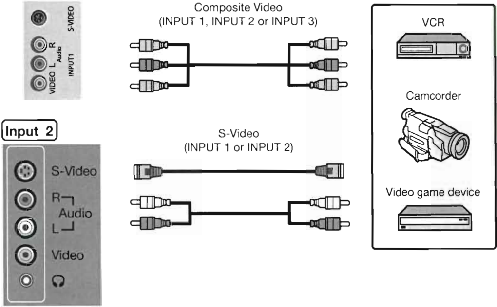
Figure 3-5. Composite and S-Video Connections
