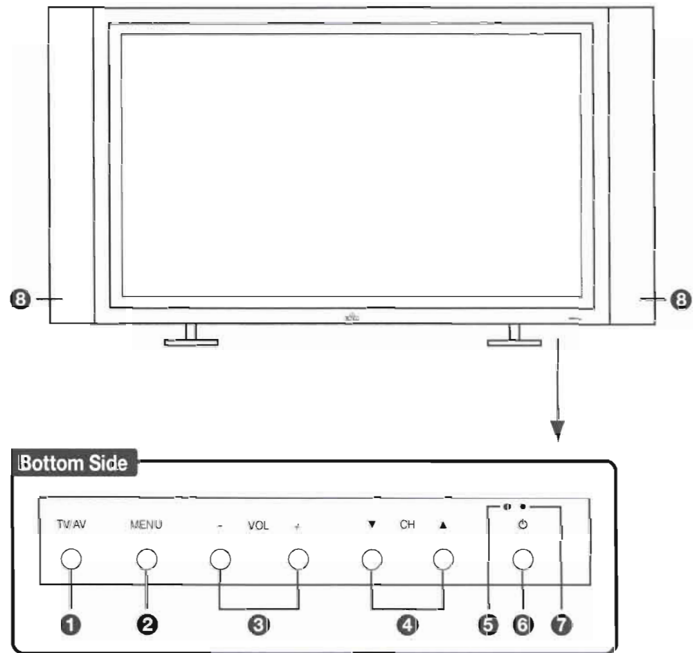
Figure 2-2. CR-32HD Controls and Indicators
