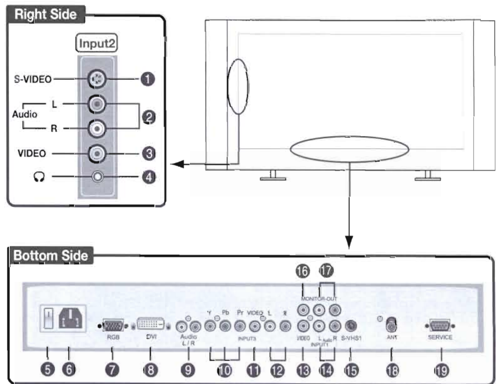
Figure 2-4. CR-32HD Rear-Panel Inputs and Outputs
