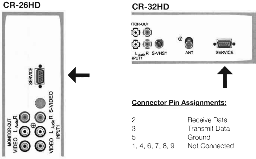
Figure 3-8. RS-232 Control System Connection
