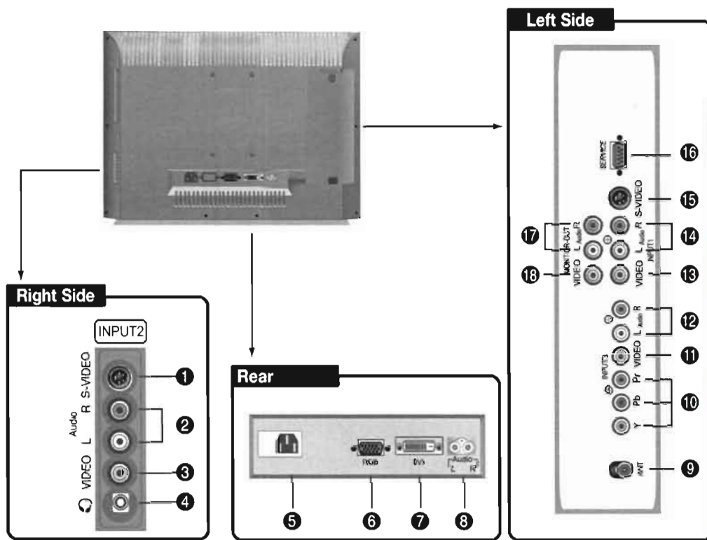
Figure 2-3. CR-26HD Rear-Panel Inputs and Outputs
