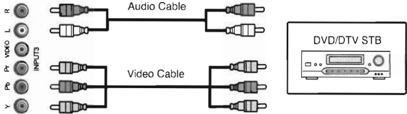
Figure 3-4. Component Video Connections
