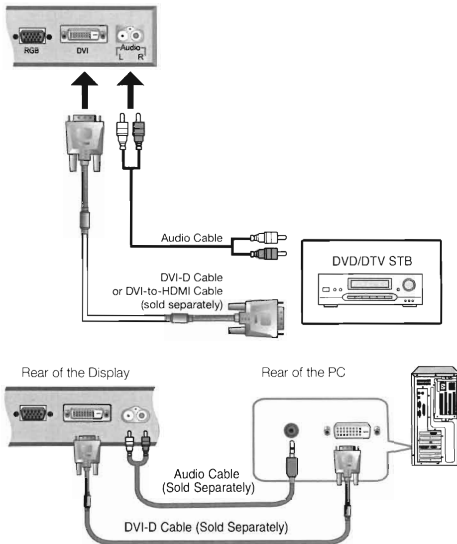
Figure 3-2. DVI Connections
