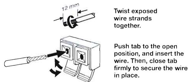
Figure 3-11. Connecting Speakers
