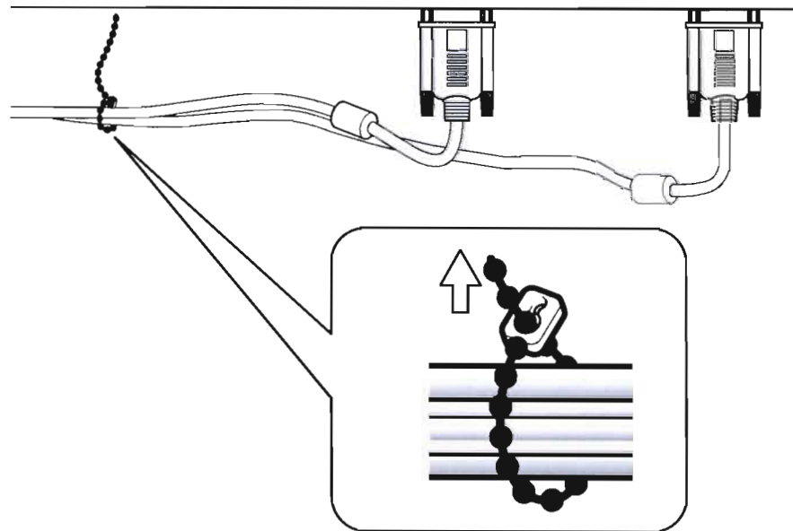
Figure 3-13. Installing the Cable Ties
