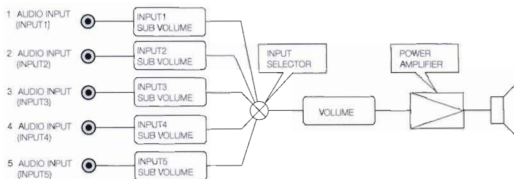
Figure 4-6. Audio System Functional Block Diagram
