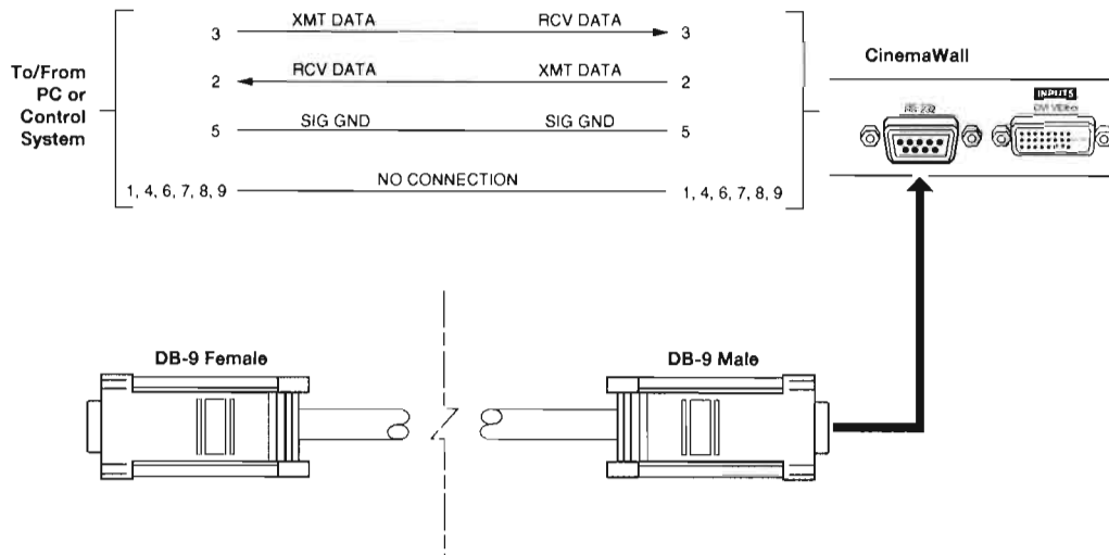
Figure 3-12. RS-232 Control System Connection
