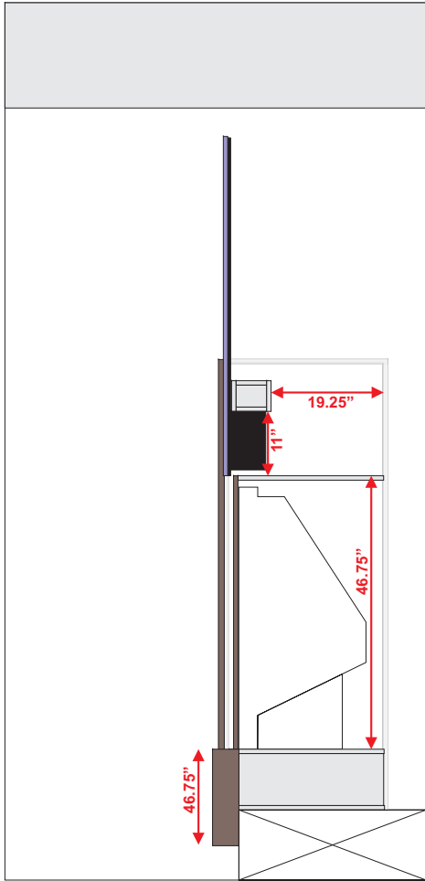
TV and Lift-up Area Side View
