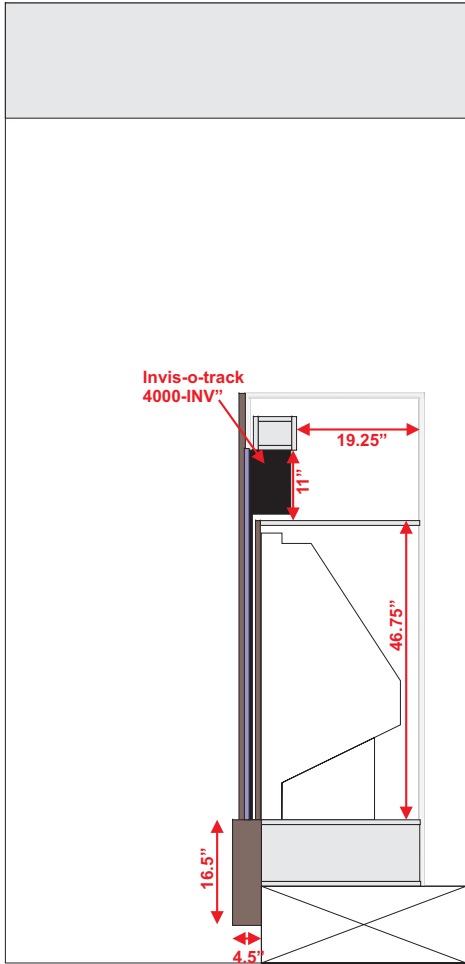
TV and Lift Area Side View
