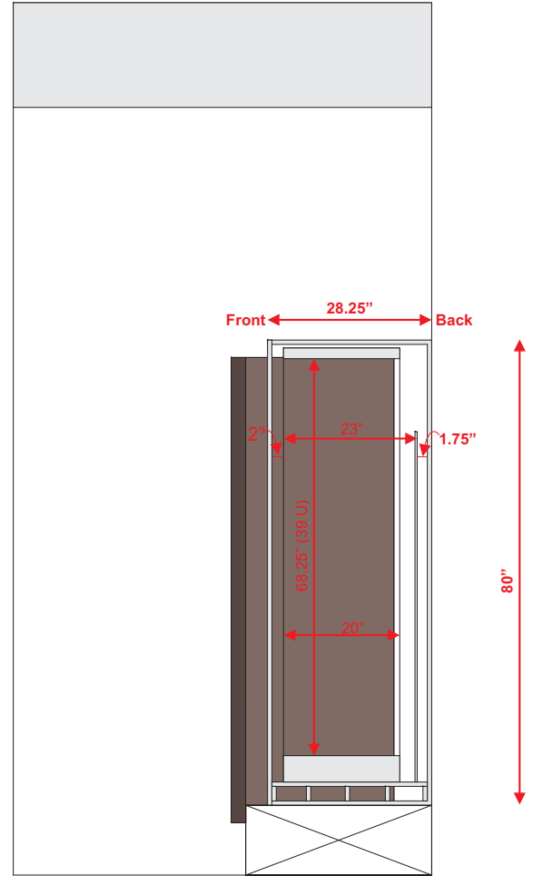
Rack Cabinet Side View
