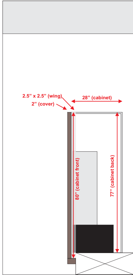
Speaker Cabinet Side View
